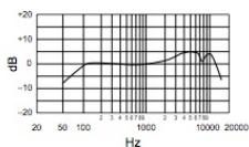
Frequency Response
